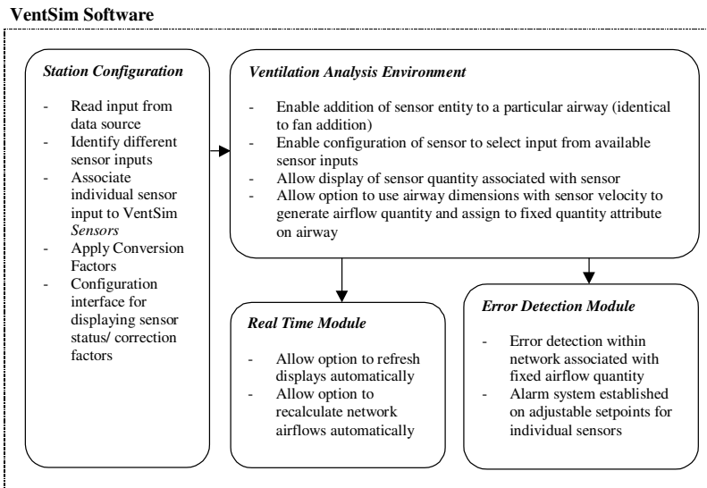
Figure 3. Ventsim Real Time Integration Modifications
