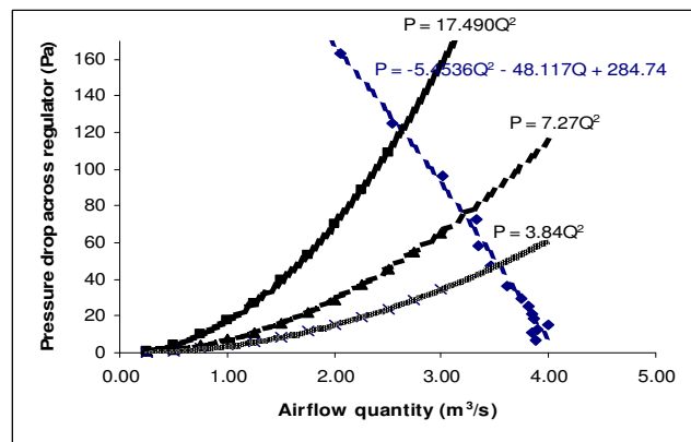
Figure 6. UQEM regulator characteristic curves.
